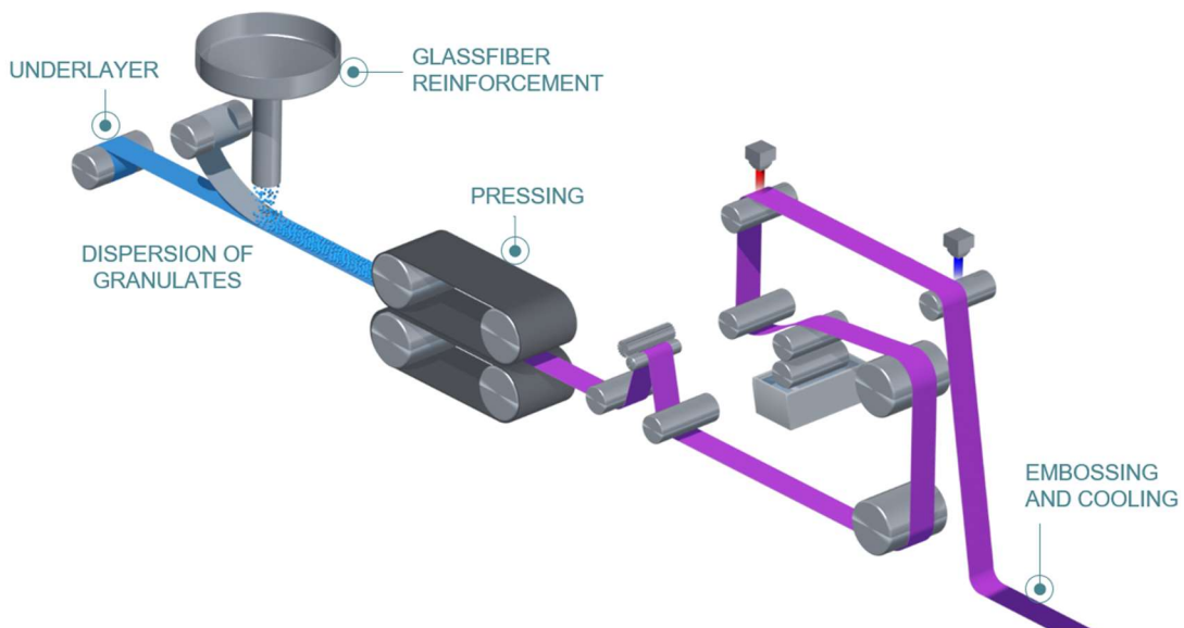
Figure 1: Pressing production process diagram
